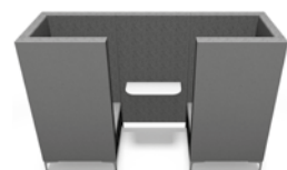
Huddle Cave Two Seater width 2380, depth 760, height 1490, seat height 440 mm
