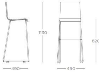
BARSTOOL - SKID FRAME JINBA.S
