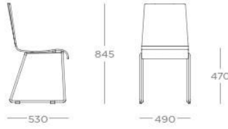
CHAIR - SKID FRAME JINDC.S
