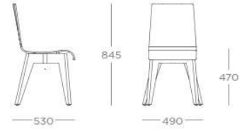
CHAIR - WOODEN FRAME JINDC.W
