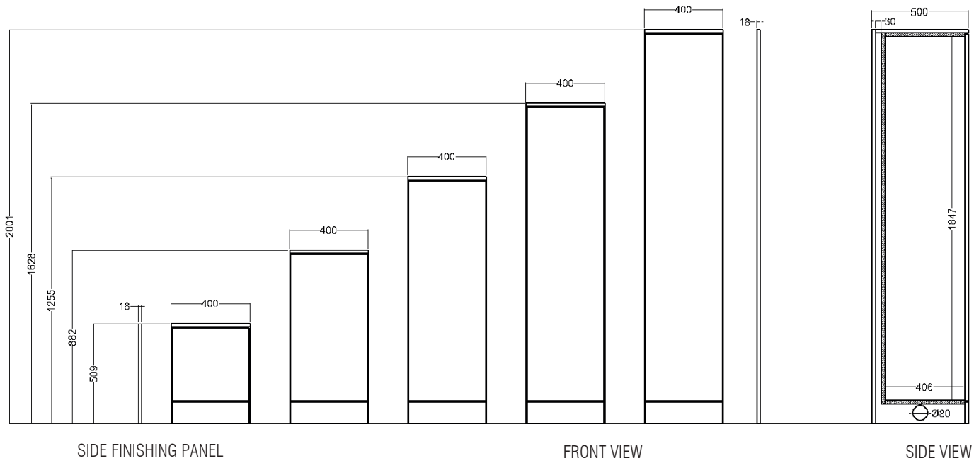
Side finishing panels will add an additional 36mm overall width to the run of lockers (18mm either side).
