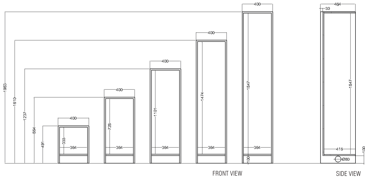
Front view showing internal and external dimensions of 1h-5h carcasses without finishing panels.
