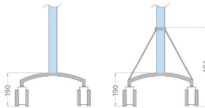
Dimensioned side view of View castor foot and View XS castor foot
